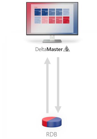
Relational
