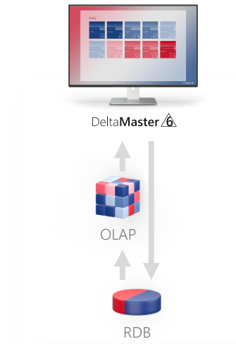
Hybrid
